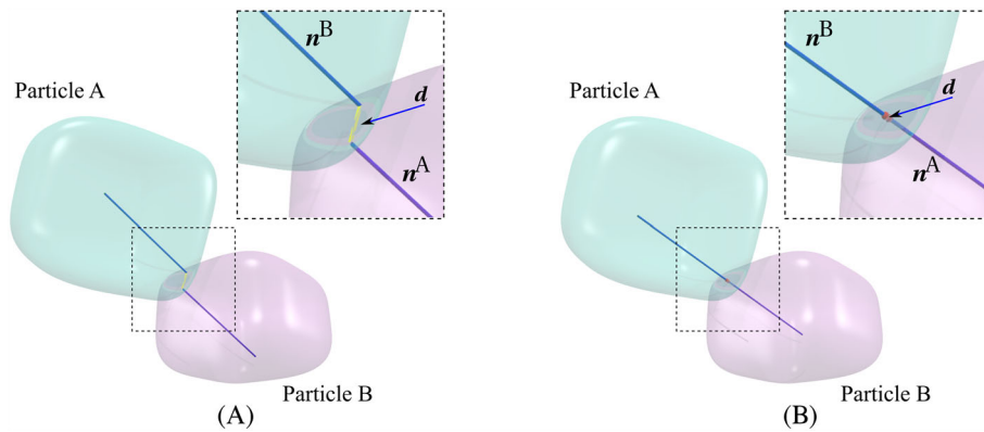
FIGURE 18 Example of two particles with a flat contact: A, the Levenberg-Marquardt (LM) algorithm fails due to slow convergence after 23 calls of the support function; B, the Gilbert-Johnson-Keerthi (GJK) algorithm succeeds after 12 calls of the support function. Note that the initial guess of the contact normal is the vector joining the mass centers of the two particles [Colour figure can be viewed at wileyonlinelibrary.com]
