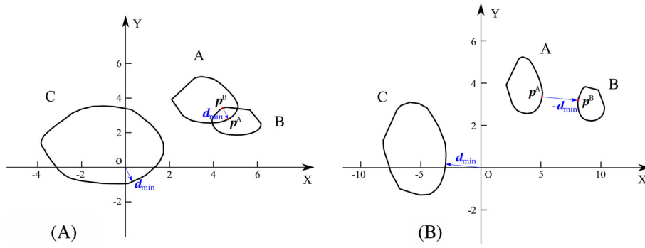
FIGURE 10 Two-dimensional schematic of Minkowski difference C of two arbitrary convex particles A and B , with or B , without contact [Colour figure can be viewed at wileyonlinelibrary.com ]
