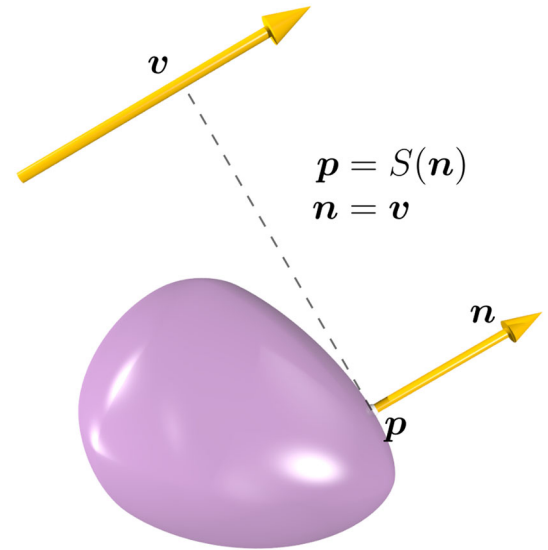
FIGURE 6 A support point \mathbf{p} on a particle surface with a given direction vector \mathbf{v} and a support function S(\mathbf{n}) . Note: \mathbf{n} is the outward normal of particle surface at the support point \mathbf{p} [Colour figure can be viewed at wileyonlinelibrary.com ]
