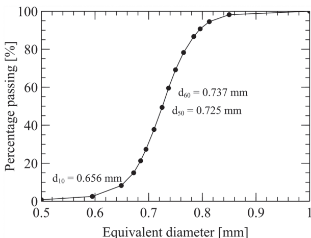
FIGURE 23 Grain size distribution of numerical specimens
