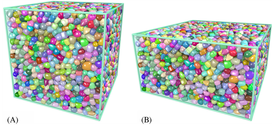
FIGURE 24 Configurations of the specimen with poly-superellipsoids at A, the initial and B, the final states. Color is for tracking particle movement intuitively [Colour figure can be viewed at wileyonlinelibrary.com ]
