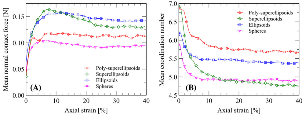
FIGURE 26 Evolution of A, mean normal contact force and B, mean coordination number for specimens with different particle shapes during shearing [Colour figure can be viewed at wileyonlinelibrary.com ]
