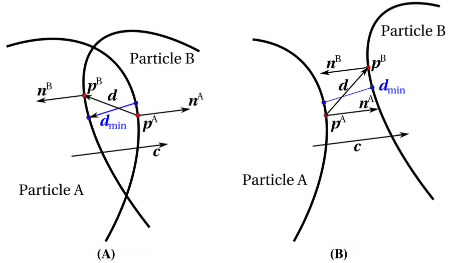
FIGURE 11 Two-dimensional schematic of the optimization solving for A, contacting and B, noncontacting particle-particle pairs [Colour figure can be viewed at wileyonlinelibrary.com]
