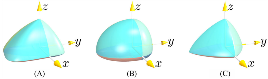
FIGURE 2 A poly-superellipsoid ( r_x^+ = 1.0, r_x^- = 0.5, r_y^+ = 0.5, r_y^- = 2.5, r_z^+ = 0.5, r_z^- = 1.7 and \epsilon_1 = \epsilon_2 = 1.0 ) in a local coordinate system with origin A, at the geometric center and B, at the mass center. Note: One color stands for one octant [Colour figure can be viewed at wileyonlinelibrary.com ]
