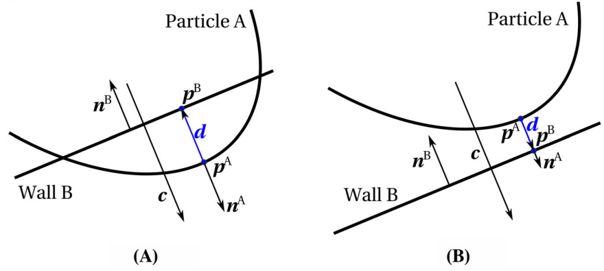
FIGURE 9 Two-dimensional schematic of the contact quantities for A, contacting and B, noncontacting particle-wall pairs [Colour figure can be viewed at wileyonlinelibrary.com ]
