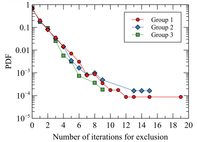
FIGURE 15 Probability distribution function (PDF) of number of iterations needing to exclude two noncontacting particles [Colour figure can be viewed at wileyonlinelibrary.com ]
