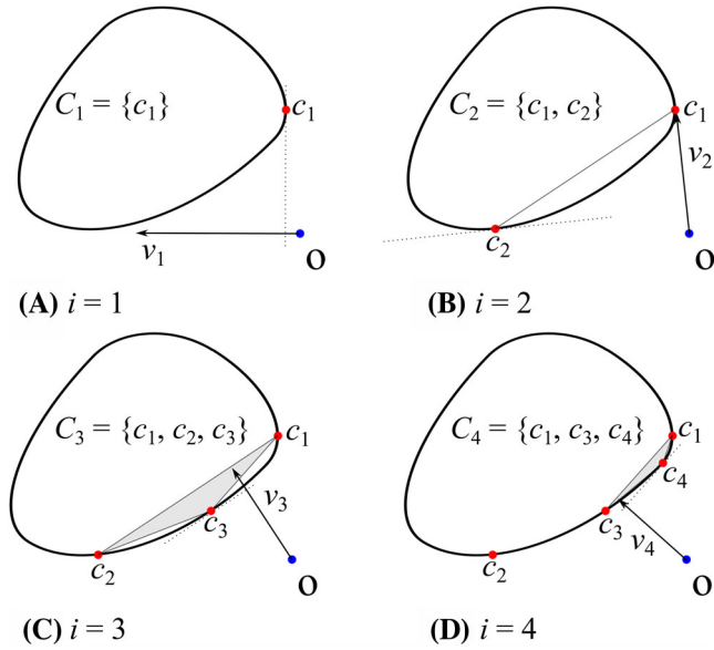
FIGURE 14 Two-dimensional illustration of Gilbert-Johnson-Keerthi (GJK) iterations for Minkowski difference not enclosing the origin [Colour figure can be viewed at wileyonlinelibrary.com]
