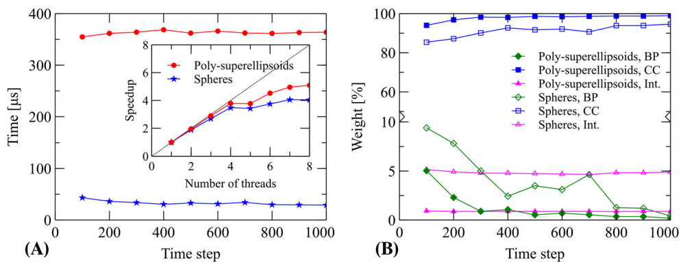
FIGURE 22 A, The single-thread computation time averaged among all interactions over every 100 time steps for poly-superellipsoids and spheres; Inset: speedup of simulations with multithreads parallelized by OpenMP; B, the weight of computation time by different discrete element method (DEM) processes for poly-superellipsoids and spheres with a single thread, BP: broad phase for contact detection; CC: contact computation including the narrow phase for contact detection and computation of contact geometry and forces; Int.: integration of particle motion [Colour figure can be viewed at wileyonlinelibrary.com ]
