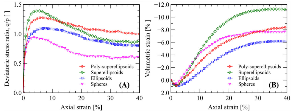
FIGURE 25 Evolution of A, deviatoric stress ratio q/p and B, volumetric strain for specimens with different particle shapes during shearing [Colour figure can be viewed at wileyonlinelibrary.com ]
