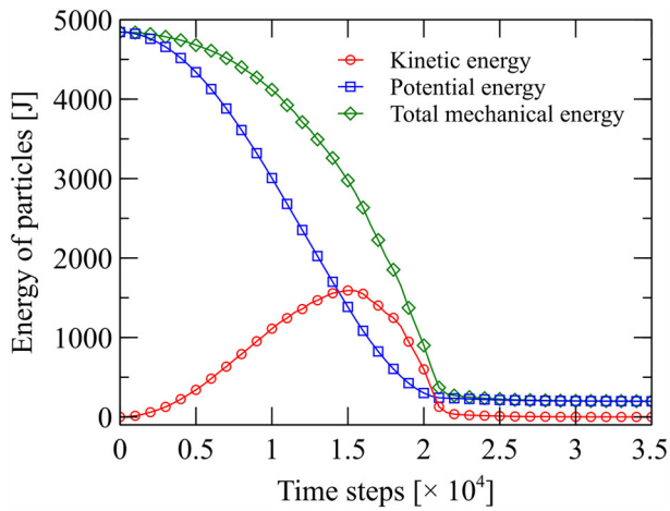
FIGURE 20 Variations of kinetic, potential, and total energy of particles during the packing [Colour figure can be viewed at wileyonlinelibrary.com ]
