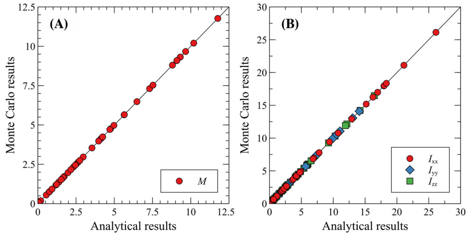
FIGURE 7 Comparison between the Monte Carlo and analytical results of A, mass and B, principal moments of inertia for 50 random poly-superellipsoids [Colour figure can be viewed at wileyonlinelibrary.com ]
