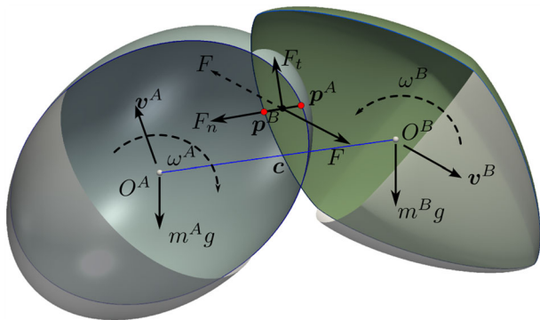
FIGURE 8 Two contacting particles with exaggerated overlap, after Zhao et al 18 [Colour figure can be viewed at wileyonlinelibrary.com]
