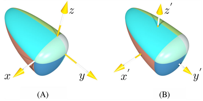
FIGURE 2 A poly-superellipsoid ( r_x^+ = 1.0, r_x^- = 0.5, r_y^+ = 0.5, r_y^- = 2.5, r_z^+ = 0.5, r_z^- = 1.7 and \epsilon_1 = \epsilon_2 = 1.0 ) in a local coordinate system with origin A, at the geometric center and B, at the mass center. Note: One color stands for one octant [Colour figure can be viewed at wileyonlinelibrary.com ]
