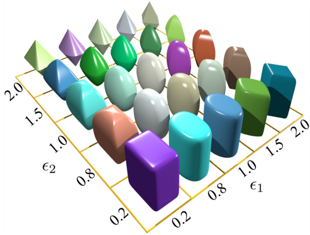
FIGURE 1 Superellipsoids with r_x = 1.0 , r_y = 1.5 , r_z = 2 and varying \epsilon_1 and \epsilon_2 [Colour figure can be viewed at wileyonlinelibrary.com ]
