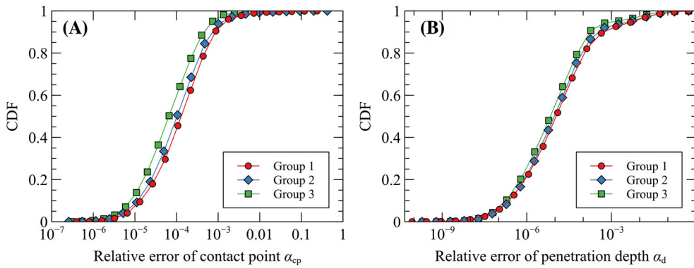
FIGURE 16 Cumulative distribution function (CDF) of relative error of A, contact point \alpha_{cp} and B, penetration depth \alpha_d [Colour figure can be viewed at wileyonlinelibrary.com]
