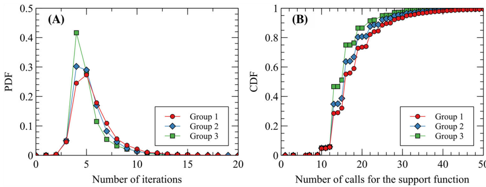
FIGURE 17 A, Probability distribution function (PDF) of number of iterations and B, cumulative distribution function (CDF) of number of calls for the support function after convergence [Colour figure can be viewed at wileyonlinelibrary.com]
