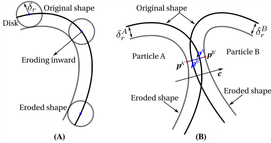
FIGURE 13 Two-dimensional schematic of A, shape erosion with a small disk (sphere in 3D) and B, two contacting particles with eroded shapes [Colour figure can be viewed at wileyonlinelibrary.com]
