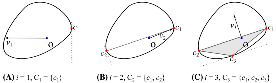
FIGURE 12 Two-dimensional illustration of Gilbert-Johnson-Keerthi (GJK) iterations for Minkowski difference enclosing the origin [Colour figure can be viewed at wileyonlinelibrary.com]
